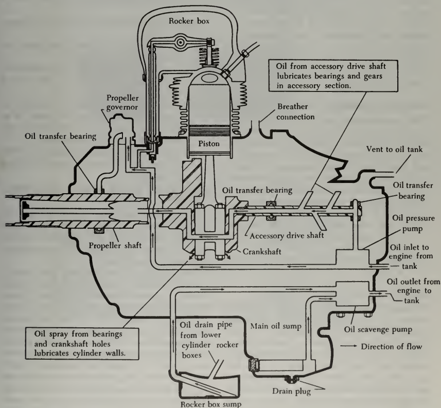
FIGURE 6-9. Schematic showing pressure dry-sump lubrication system.
